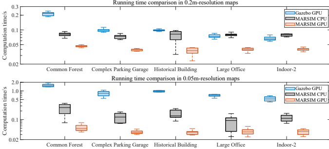
Fig. 7: Time consumption for rendering one Livox AVIA scan on a light-weight computation platform (NUC).
