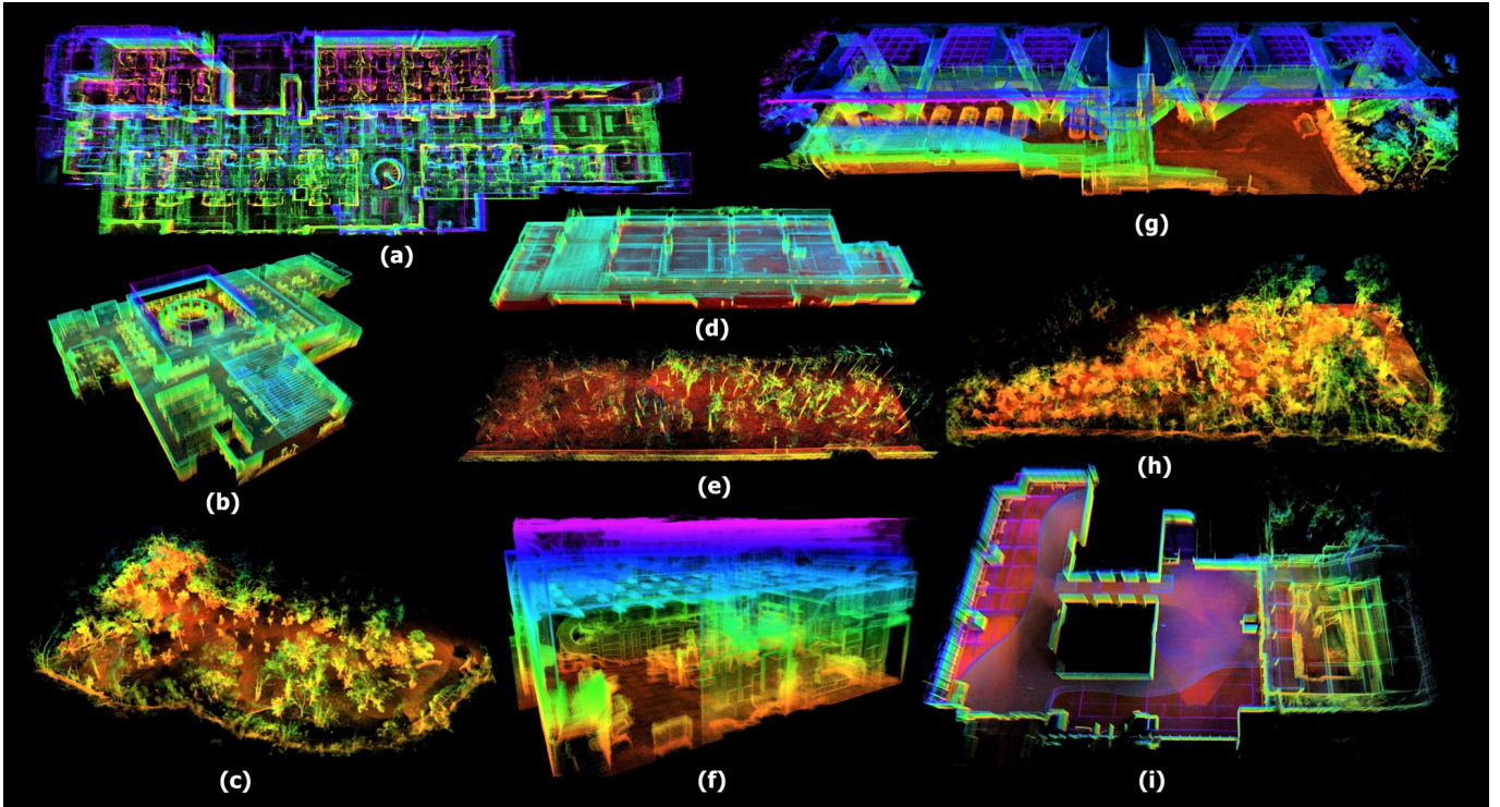
Fig. 5: High-resolution point cloud maps provided by the simulator with detailed information shown in Table I.
