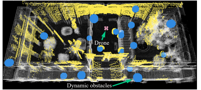
Fig. 11: Dynamic obstacles simulation in the historical building map. The blue balls are the dynamic obstacles, the yellow point clouds are the points scanned by a VLP-32 LiDAR.
