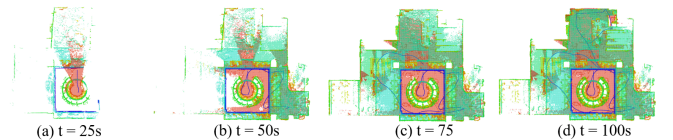
Fig. 13: Demonstration of a UAV autonomous exploration simulation in indoor-2 map, utilizing FUEL algorithm. The area scanned by the UAV after different executing times are shown.
