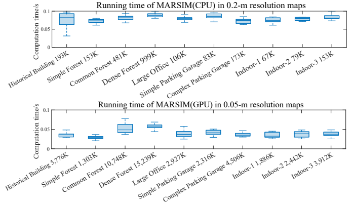
Fig. 8: Time consumption for rendering one Livox AVIA scan on all 10 realistic point cloud maps. The X-axis labels the name and size of the point cloud map.
