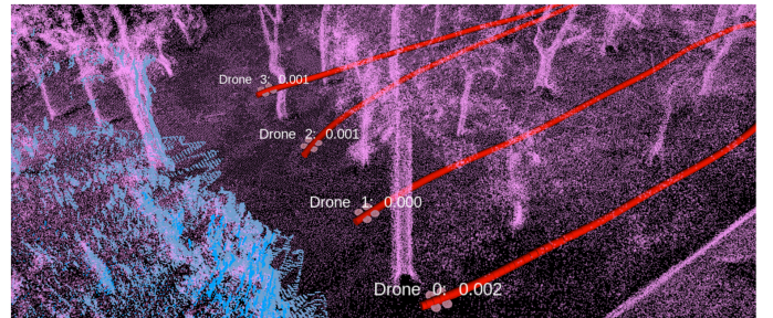
Fig. 12: Multi-UAV planning simulation. The pink models are the UAVs, and the red curves are the trajectories of the drones, avoiding the obstacles of a realistic forest map.
